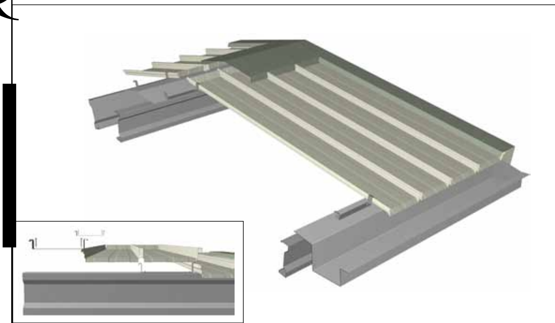
TACDECK junta alzada / viga vertical
