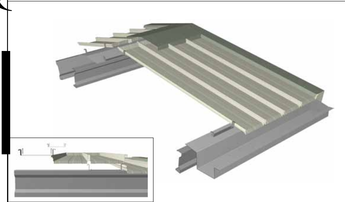
TACDECK joint debout / standing seam
