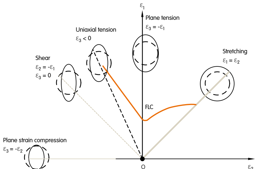
Strain diagram for sheet forming, showing a typical forming limit curve (FLC) for steel
