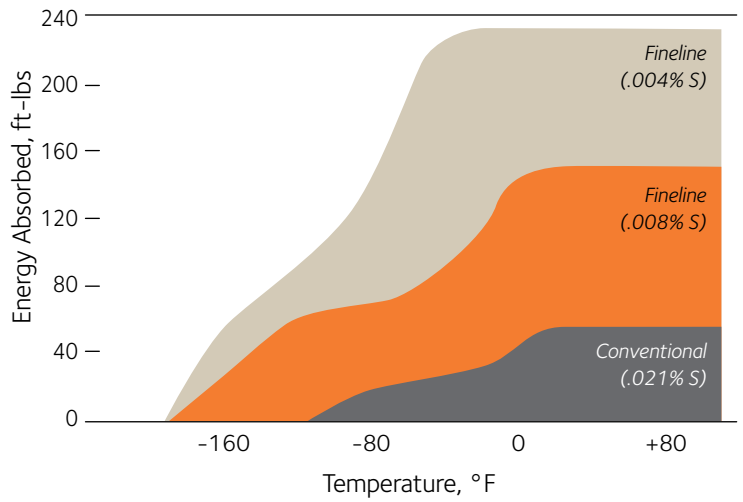
Figure 4 Comparison of Charpy V-Notch Energy Absorption for Normalized 1 – 2" Thick ASTM A633C Plates, Transverse Orientation
