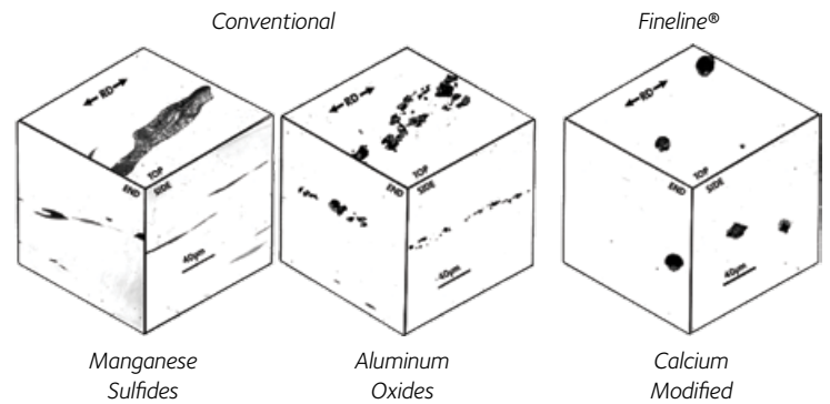
Figure 2 Inclusions in Structural Plate Steels
