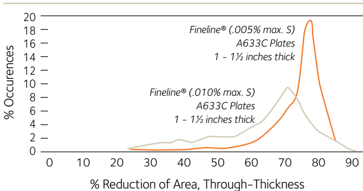
Figure 3 Distribution of Through-Thickness Reduction of Area
